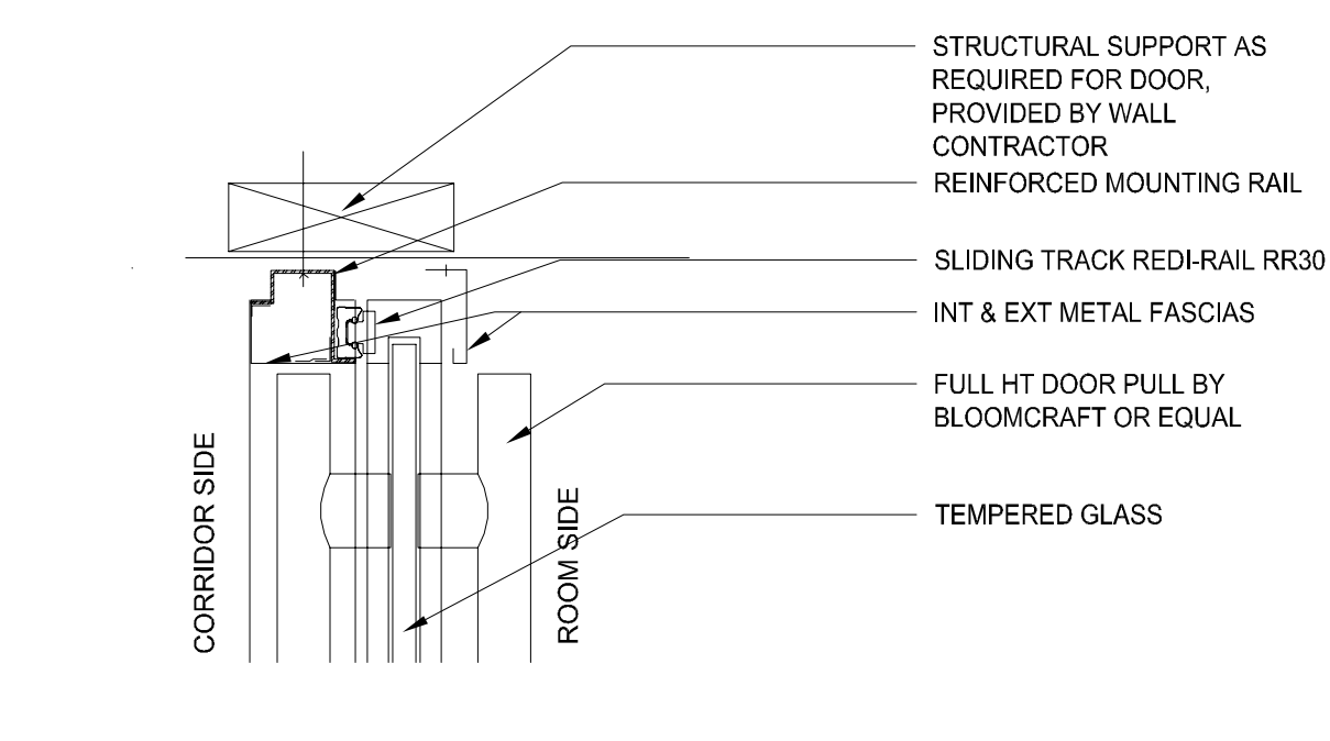
48 HEAD DETAIL SLIDING DOOR 1/5
