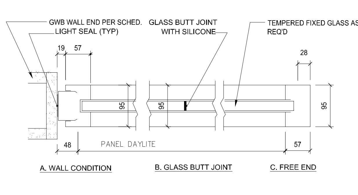
54 JAMBS DETAIL GLASS WALL 1/5
