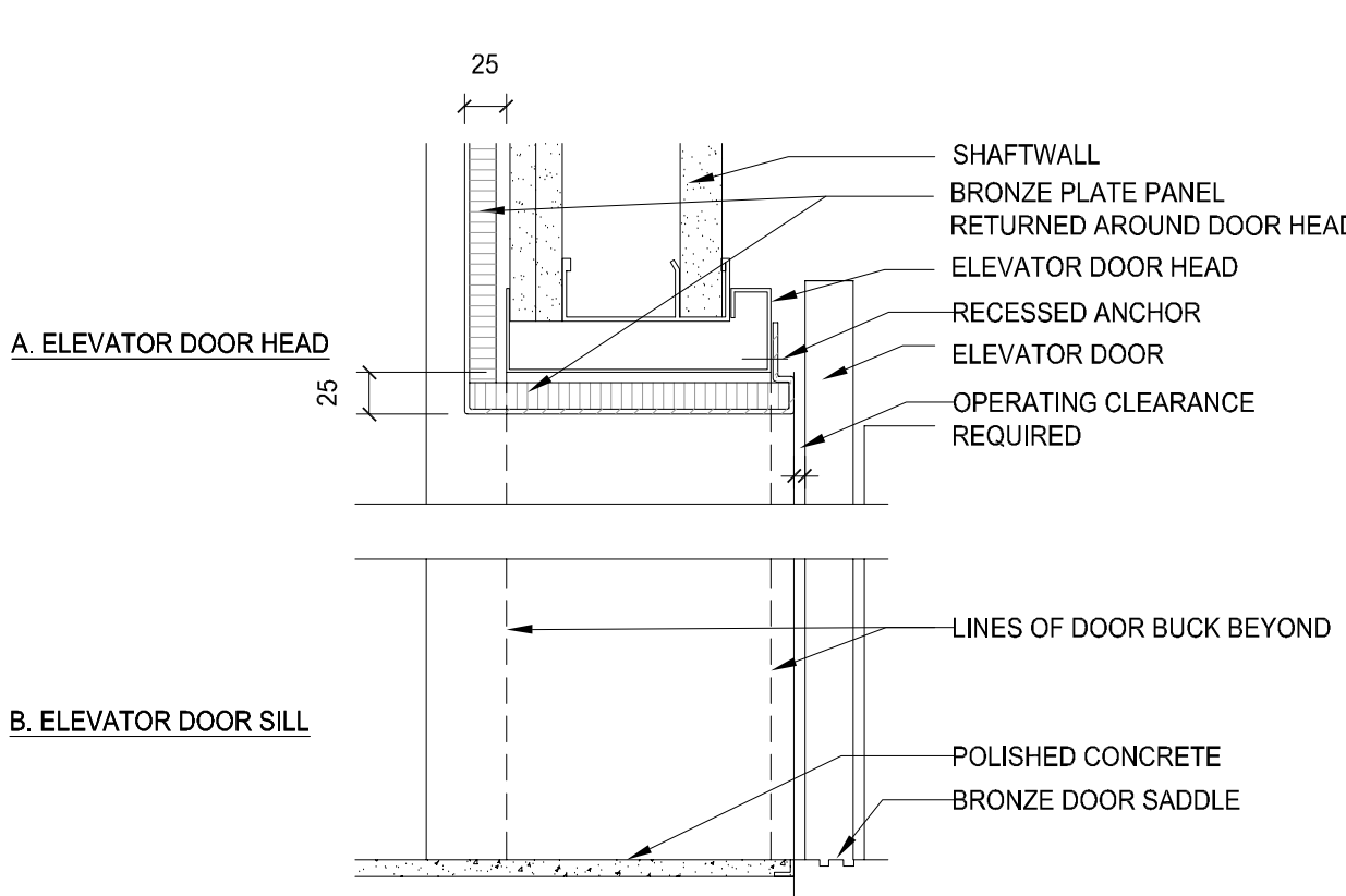
56 HEAD AND SILL DETAIL ELEVATOR DOOR BUCK 1/5
