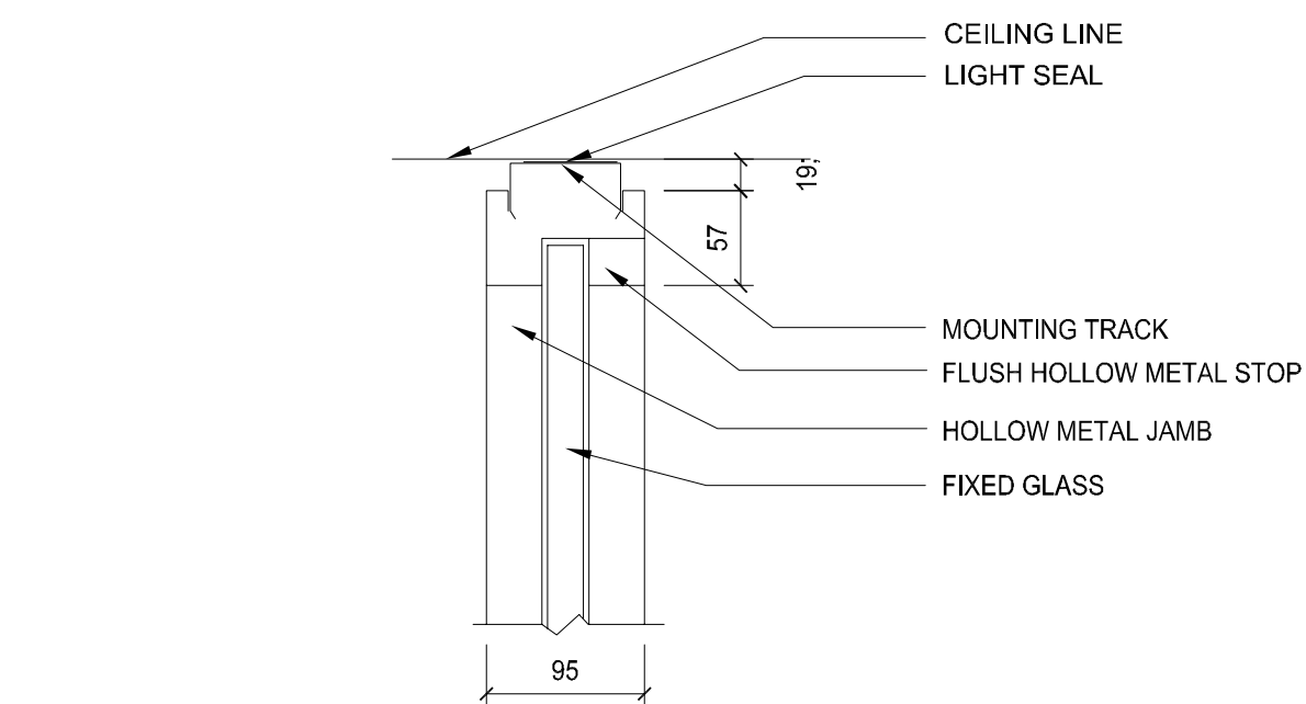
40 HEAD DETAIL FIXED GLASS WALL PANEL 1/5
