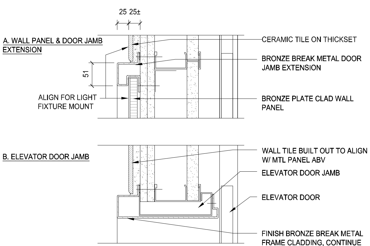
57 JAMB AND TRANSOM DETAIL ELEVATOR DOOR BUCK 1/5
