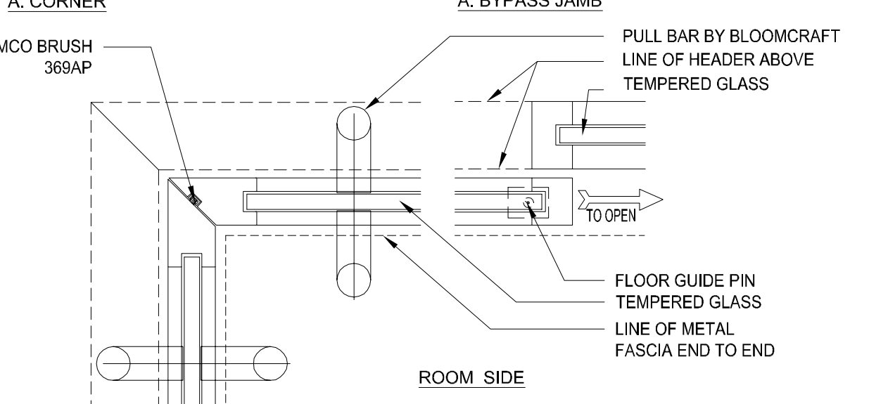
55 JAMBS DETAIL CORNER CLOSING SLIDER 1/5
