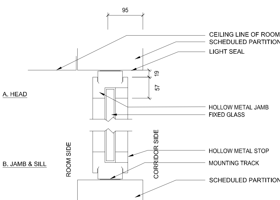
44 HEAD, SILL & JAMB FIXED GLASS WINDOW 1/5
