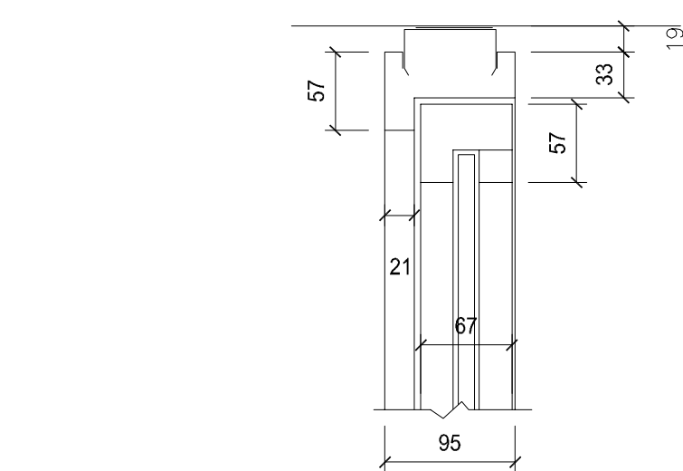
42 HEAD DETAIL HINGED DOOR 1/5
