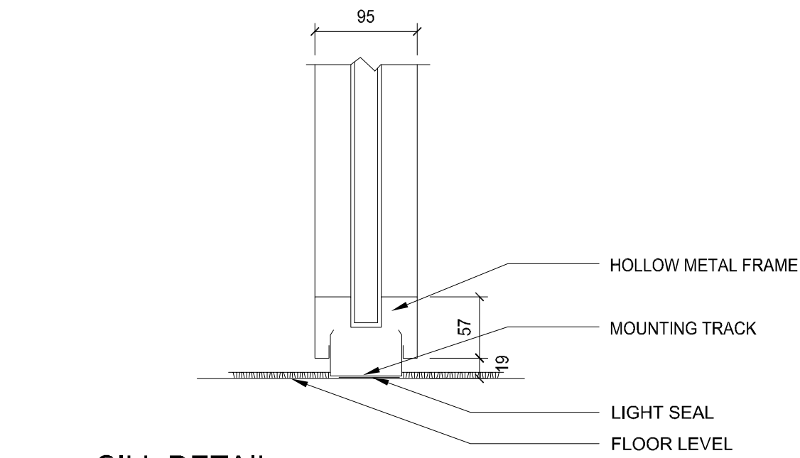
41 SILL DETAIL FIXED GLASS WALL PANEL 1/5
